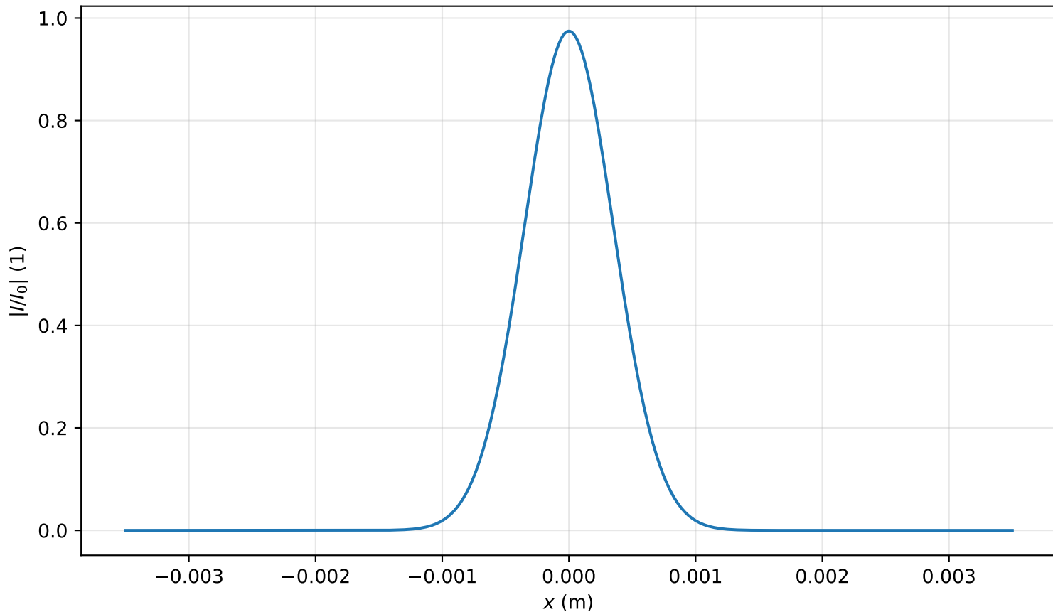
Intensity profile I(x, y = 0, z = 0.398m)/I_0 , P_{in}=0.1P_{cr} , artificial time
